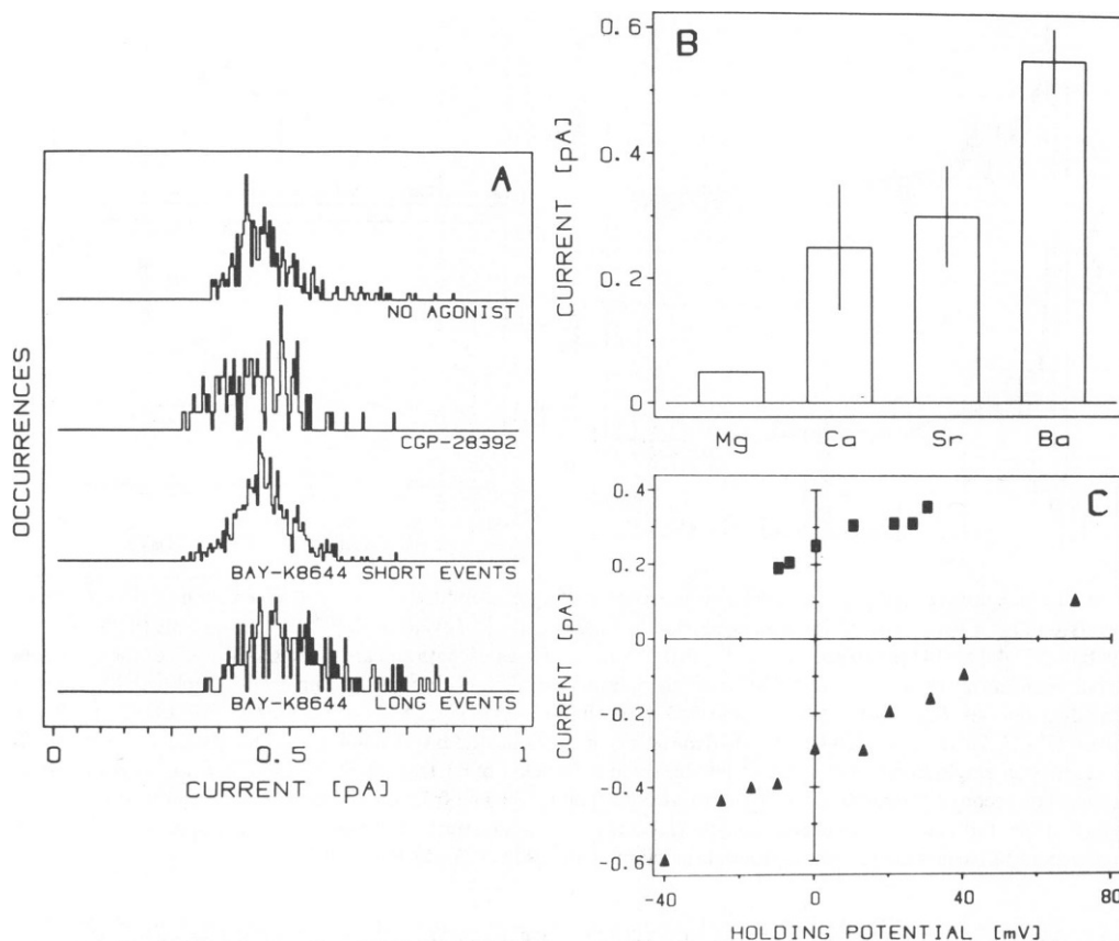
FIGURE 3 Amplitude distribution, divalent cation permeation, and reversal potential of Bay-K8644-induced single calcium channels. (A) Amplitude distribution of open channel currents at HP = 0 mV in trans 0.05 M NaCl- cis 0.05 M NaCl + 0.1 M BaCl 2 in the absence or presence of cis 3 \mu M Bay-K8644 or cis 3 \mu M CGP-28392. Events without agonist ( n = 230 ) or CGP-28392 ( n = 140 ) correspond to total openings > 20 ms. Short events in Bay-K8644 ( n = 480 ) are from the duration interval 20 \text{ ms} < t < 50 \text{ ms} and long open events ( n = 200 ), from the interval 200 \text{ ms} < t < 1,000 \text{ ms} . (B) Bar histogram of mean and standard deviation of open channel currents (events > 20 ms) at HP = 0 mV measured in trans 0.05 M NaCl; cis 0.05 M NaCl + 0.1 M XCl 2 (X = Ba ++ , Sr ++ , Ca ++ , or Mg ++ ), cis 5 \mu M Bay-K8644. Mg ++ currents cannot be measured accurately; the bar (0.05 pA) is an estimated upper limit. (C) reversal potential of single channel currents under bionic trans 0.05 M NaCl- cis 0.05 M BaCl 2 (filled squares) or trans 0.05 M BaCl 2 - cis 0.05 M NaCl (filled triangles). Reversal potential for this latter condition is +58 mV. All solutions were buffered with 0.1 mM EGTA and 10 mM Hepes-Tris, pH 7.0.
